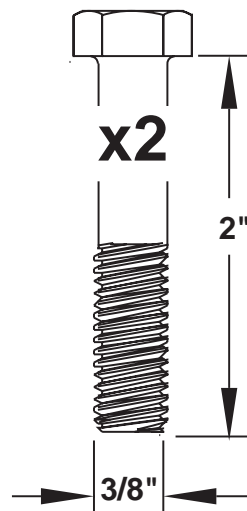
3/8" HEX BOLT
